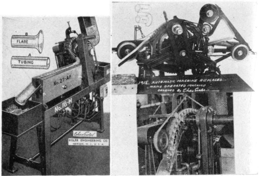
Left: The Eisler automatic flange machine, with a view of the flare and tubing. Right: The Eisler automatic flange machine ( below at close range), designed by Eisler in Hungary as the first of its kind and made by Eisler for Westinghouse in 1915. (Patent No. 1,635,316.) Its outstanding feature was the perpetual chain drive for turning the glass tubing.
